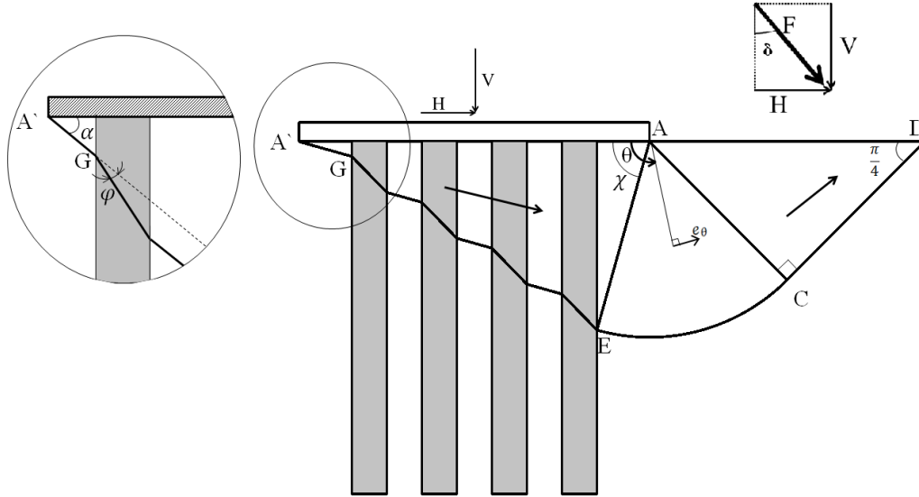
Figure 7. Generalized Prandtl type failure mechanism I
