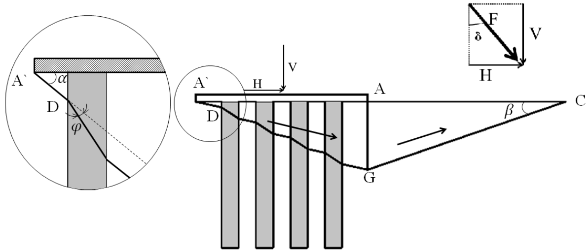
Figure 8. Two translational zones failure mechanism II
