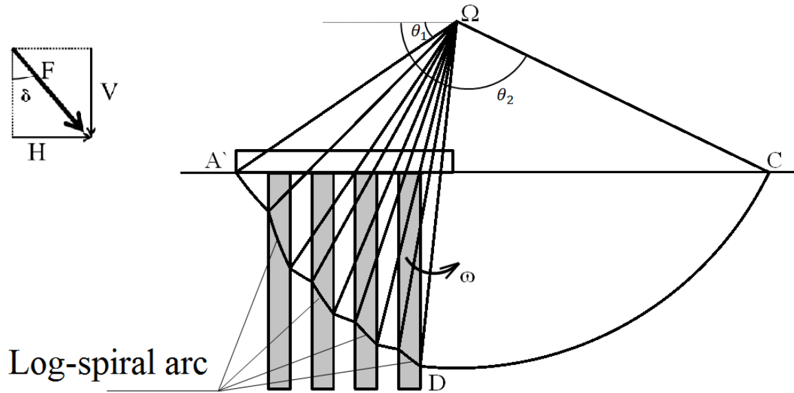
Figure 9. Rotational failure mechanism III
