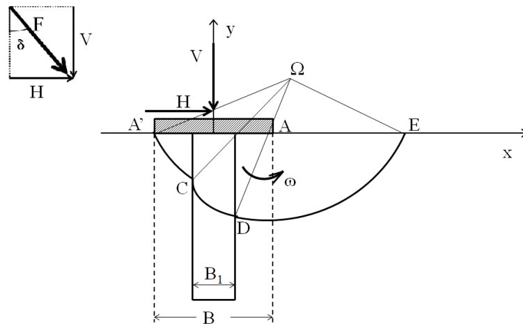
Figure 6. Rotational failure mechanism III
