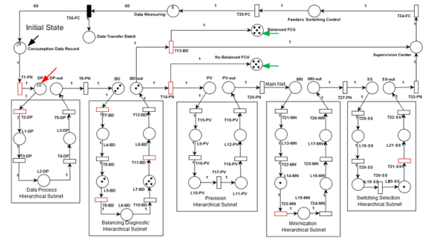
Figure 5: DPMS THPN Simulation.
