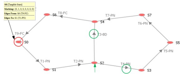
Figure 4: Main DPMS Reachability Graph with initial marking.
