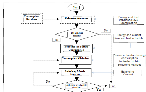
Figure 2: DPMS flowchart.
