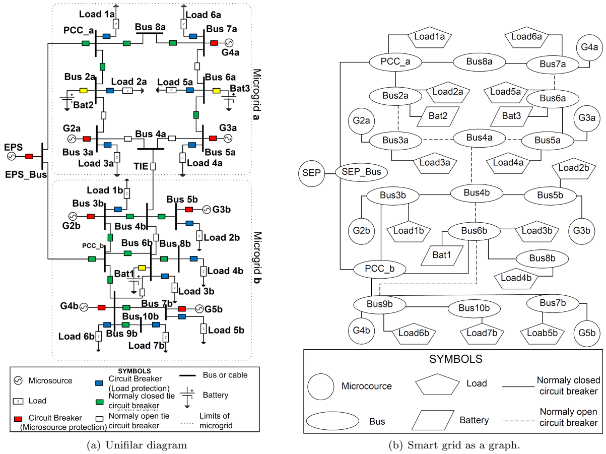
Figure 2: Representations of grid under study
