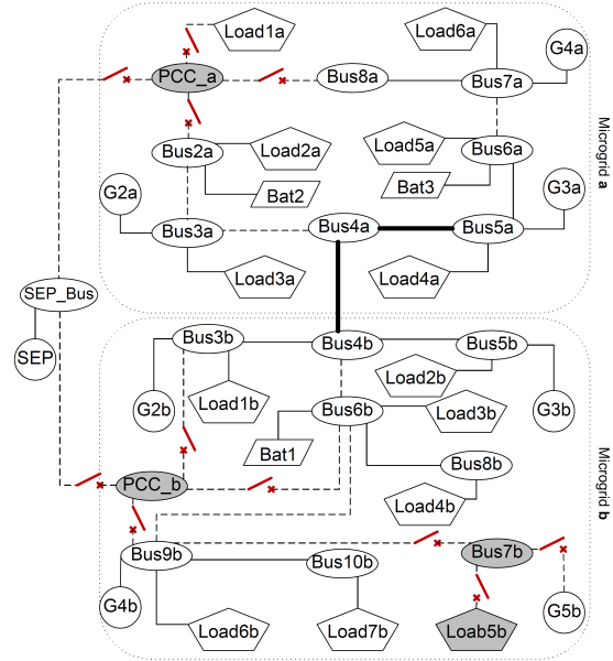
Figure 4: Smart grid in reconfiguration state after failure in PCC_b , Bus7b and PCC_a ( Scenario 5 ).
