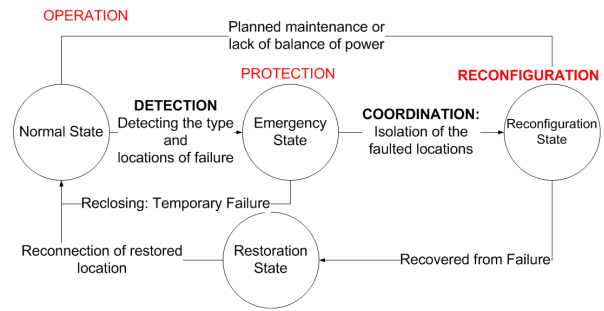
Figure 1: State diagram of the smart grid system.
