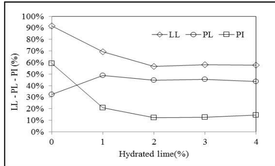
Figure 4. Atterberg limits variation with hydrated lime content.
