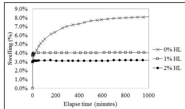
Figure 5. Evolution of swelling with time in centrifuge test.
